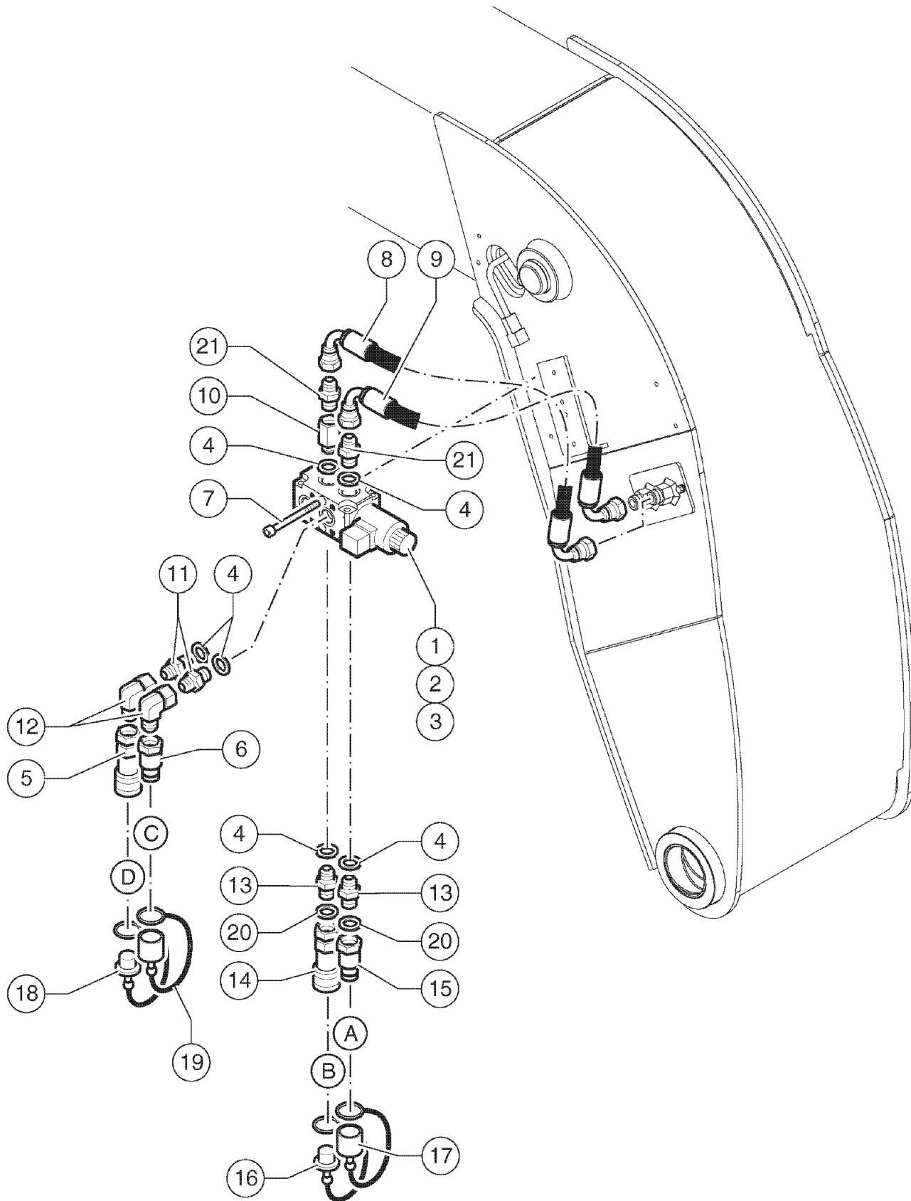
619.1 610027 Auxiliary Hydraulic Line, View 1
