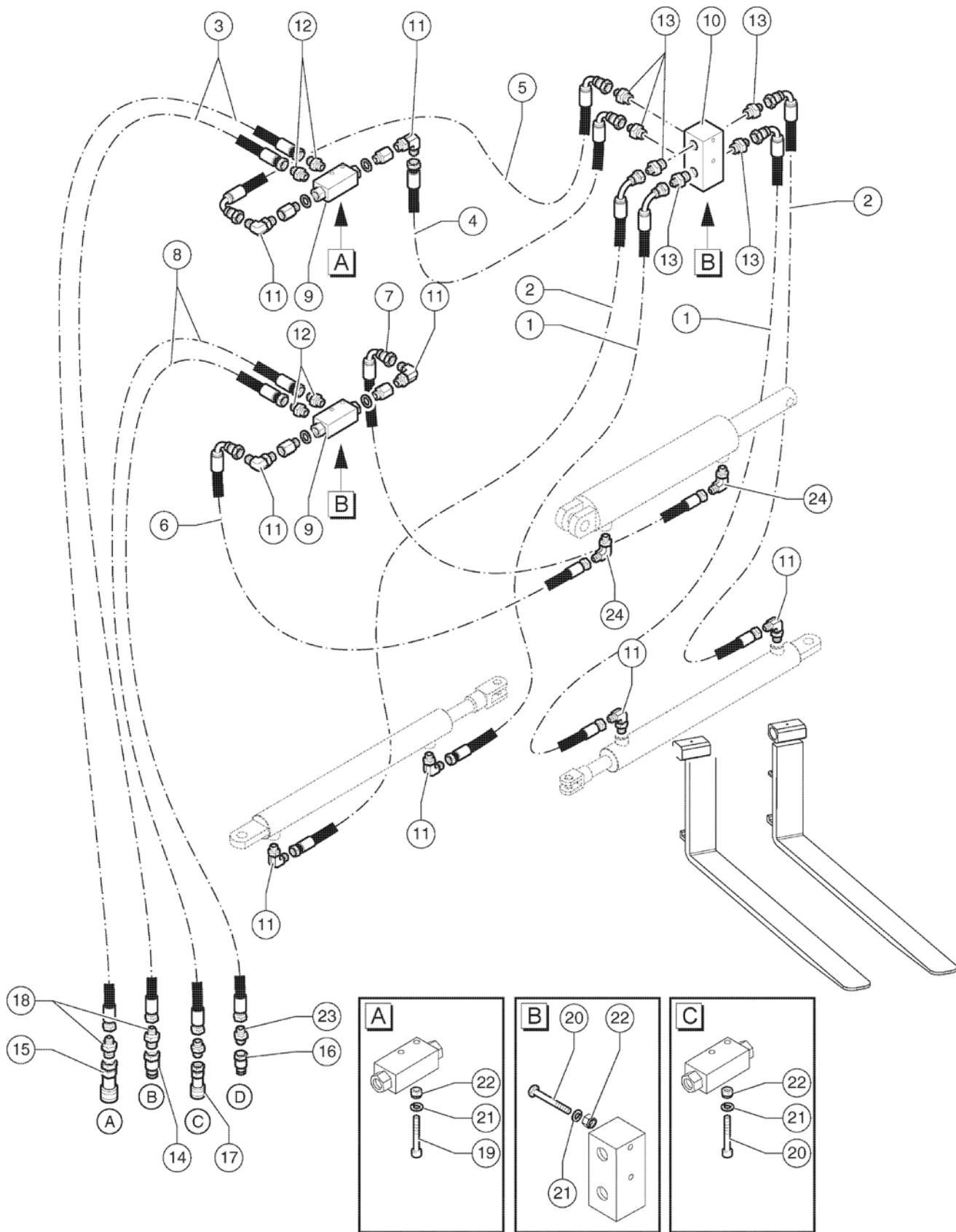
620.1 610028 Auxiliary Hydraulic Line, View 2
